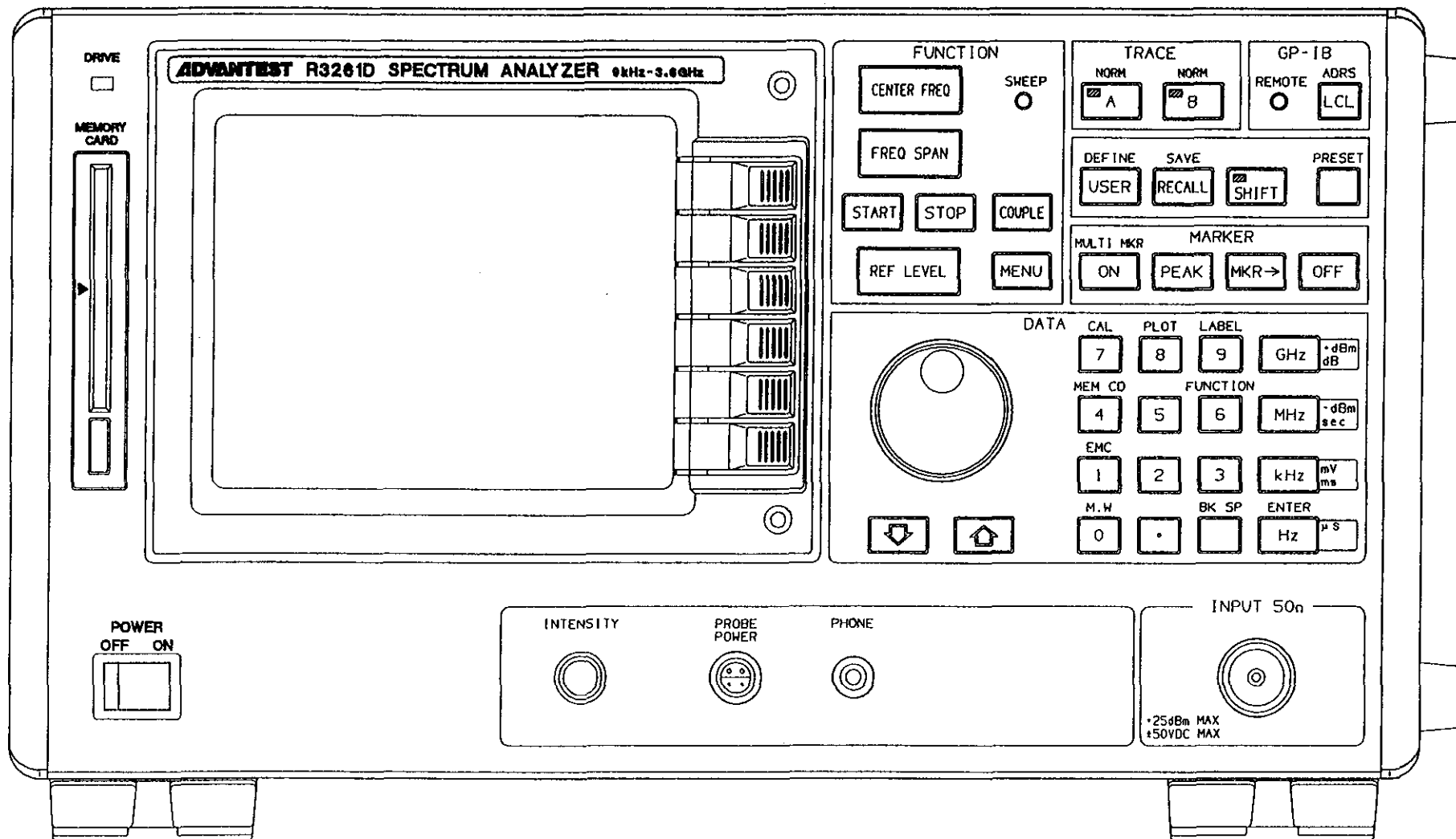
R3261D FRONT VIEW
