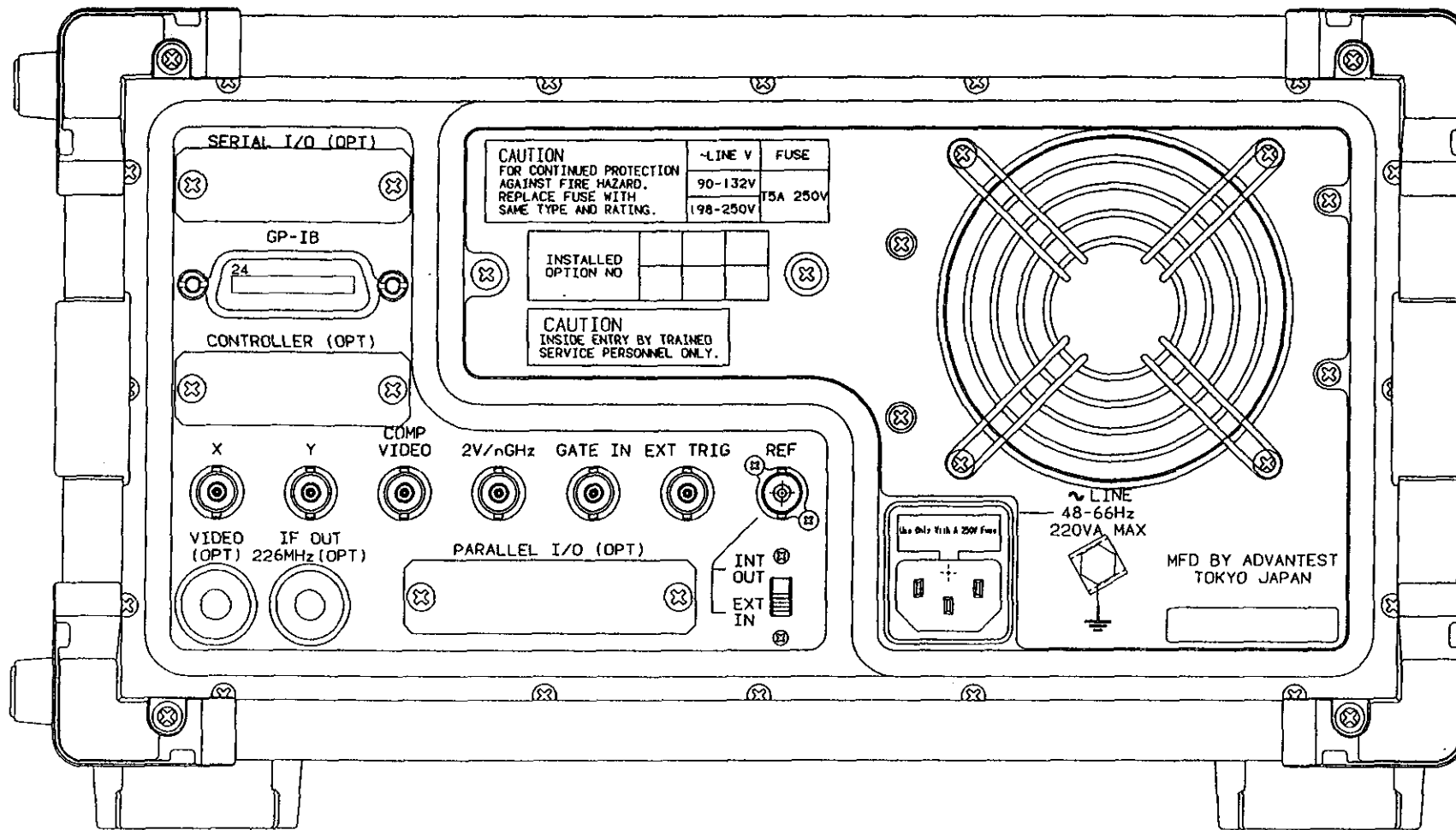
R3261/3361 SERIES REAR VIEW (Standard)
