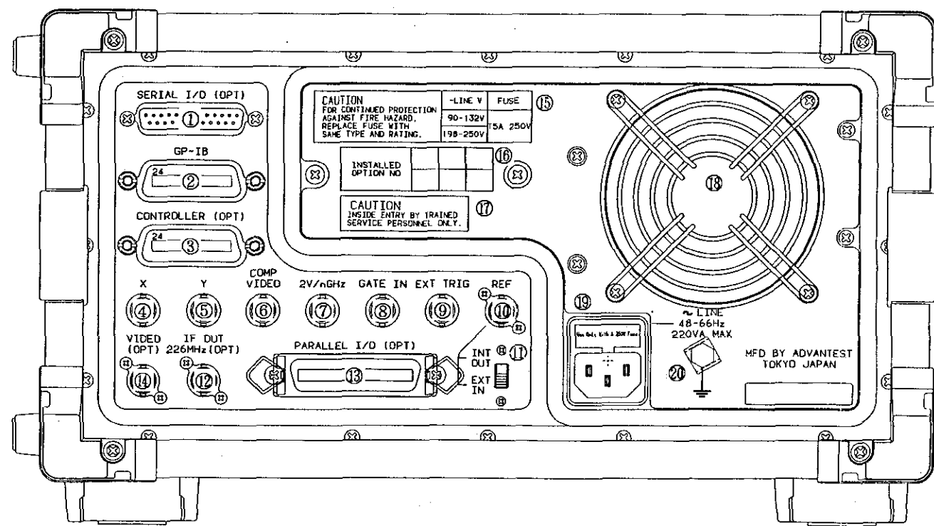
Figure 2 - 2 Rear Panel
