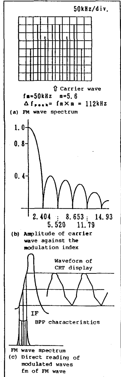
Figure 6 - 4 FM Signal
