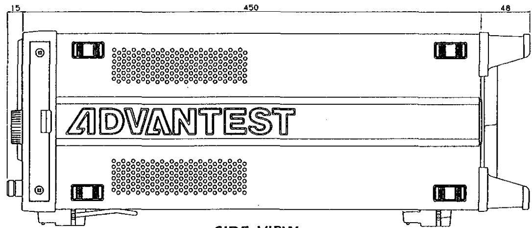
SIDE VIEW
