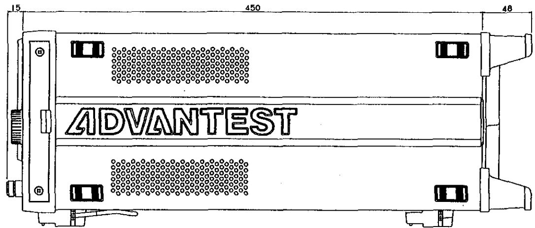
SIDE VIEW
