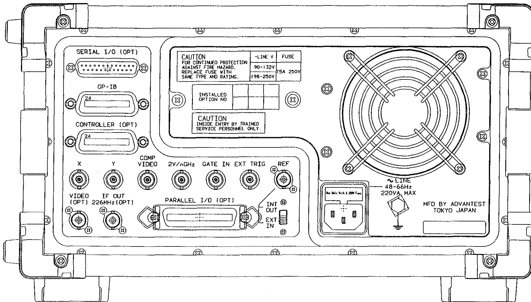
R3261/3361 SERIES REAR VIEW (When option is installed)
