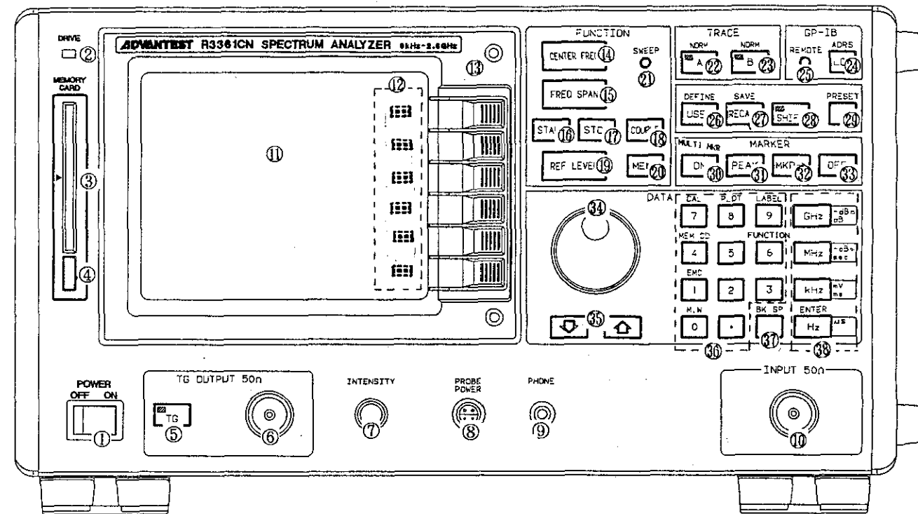
Figure 2 - 1 Front Panel
