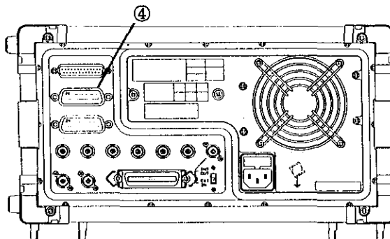
Rear panel
