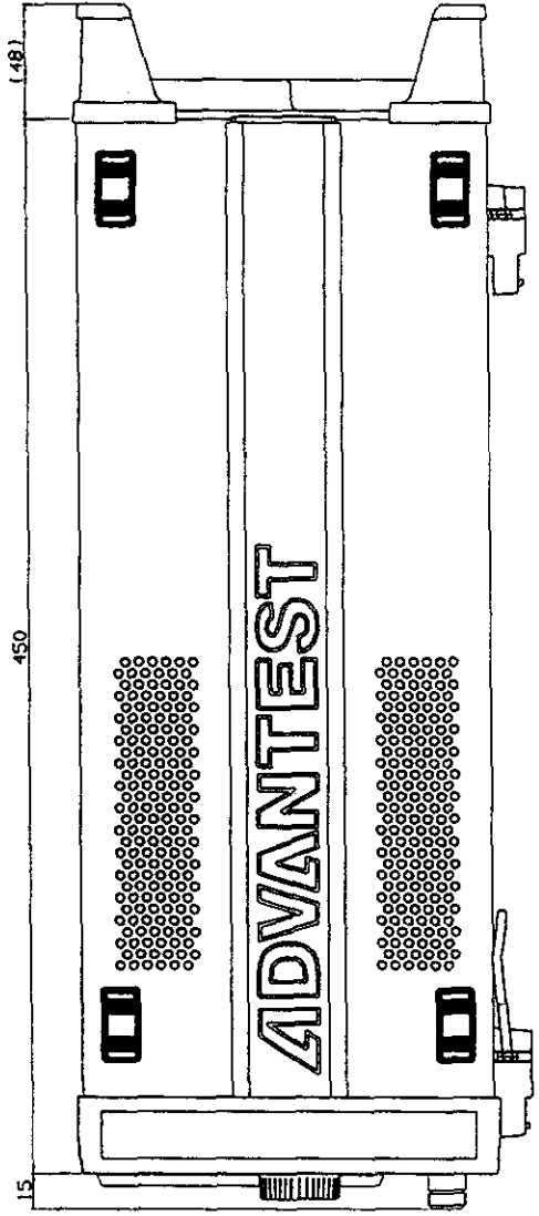
SIDE VIEW
